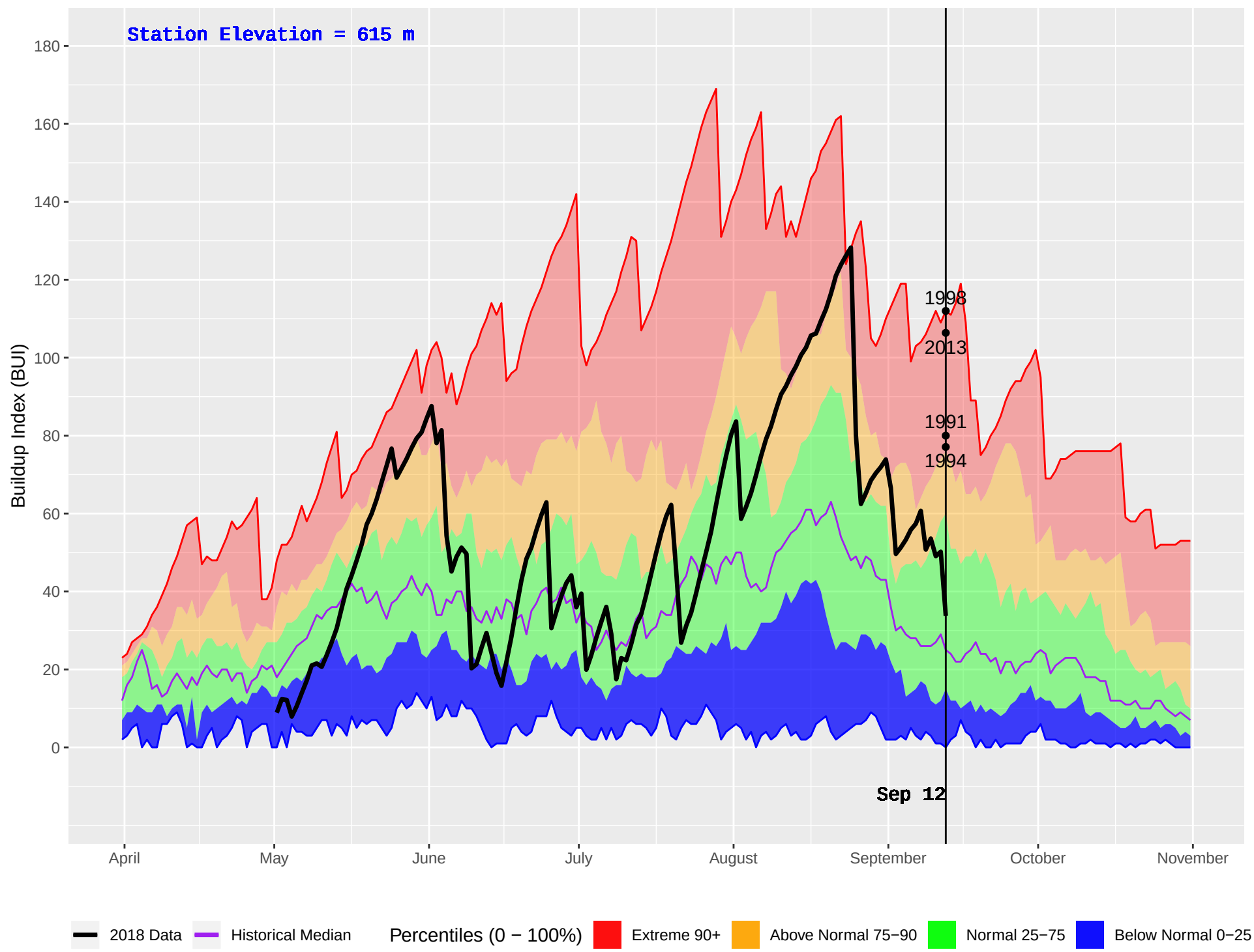
HIXON (187) : Historical (1976–2016) and Current (2018) Daily Buildup Index (BUI)
