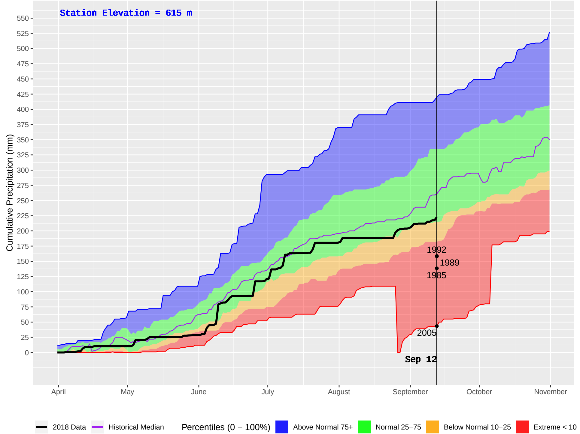
HIXON (187) : Historical (1976–2016) and Current (2018) Daily Cumulative Precipitation
