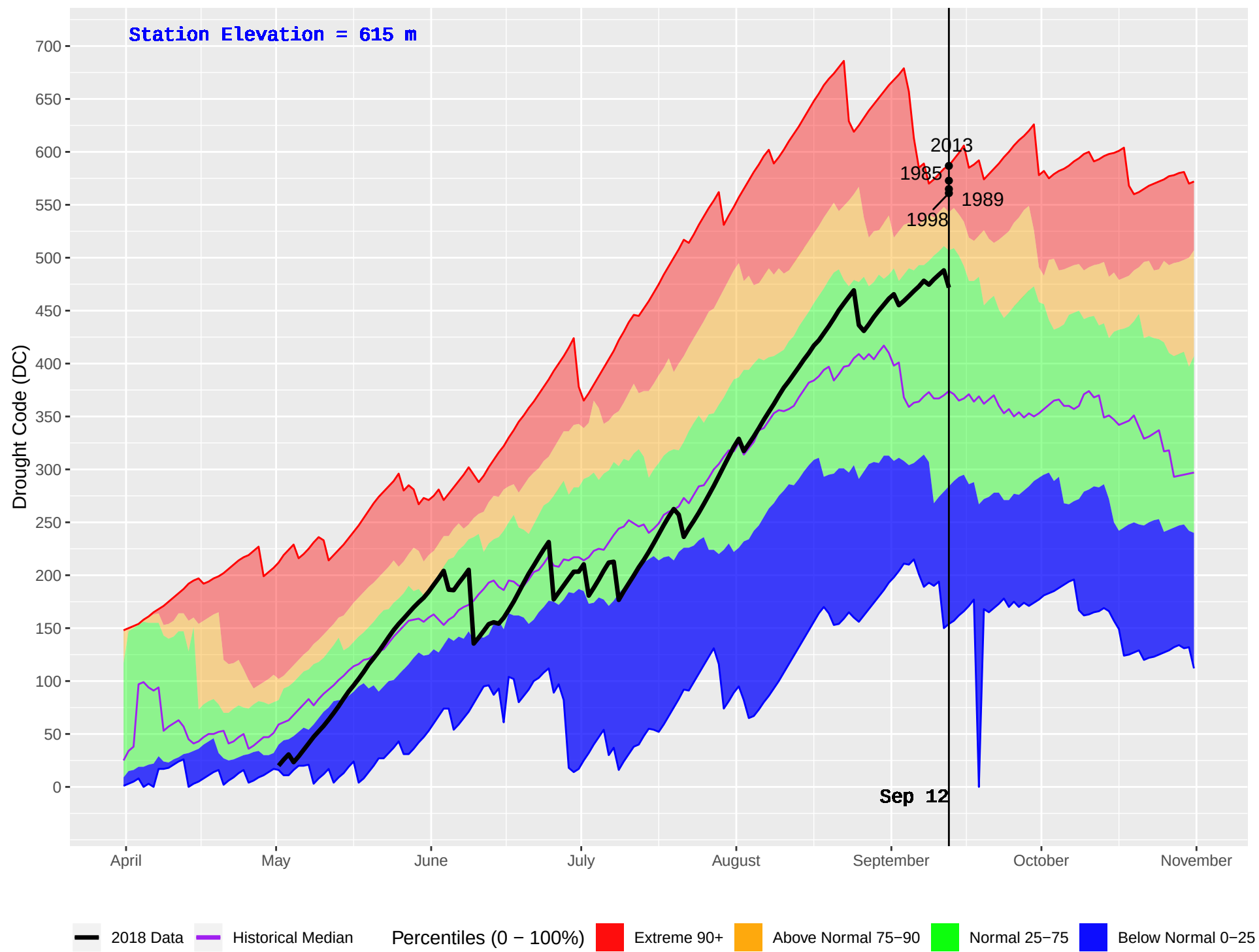
HIXON (187) : Historical (1976–2016) and Current (2018) Daily Drought Code (DC)
