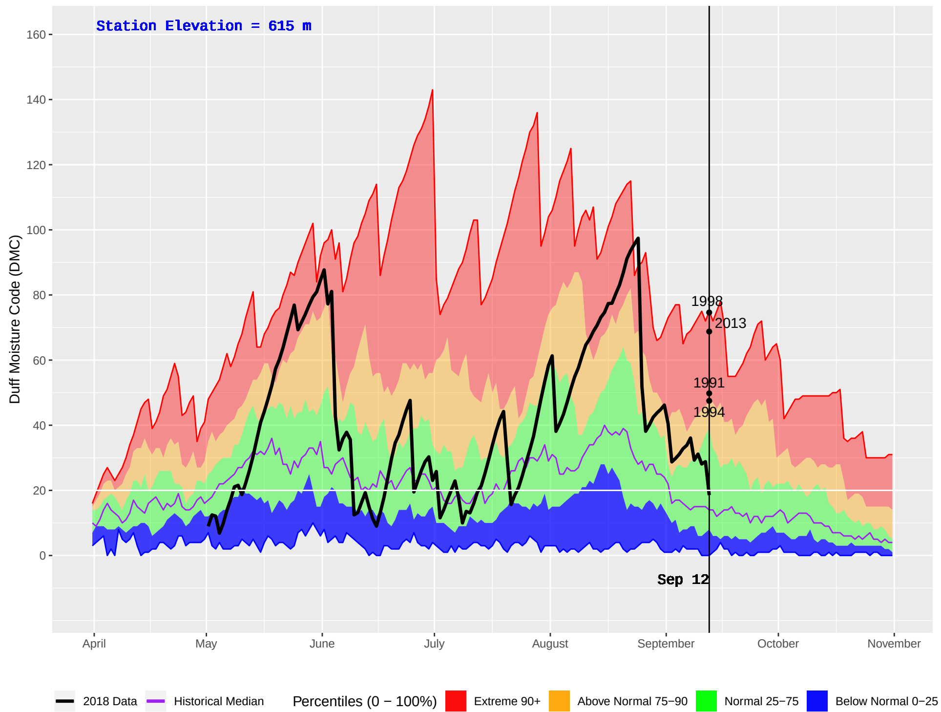
HIXON (187) : Historical (1976–2016) and Current (2018) Daily Duff Moisture Code (DMC)
