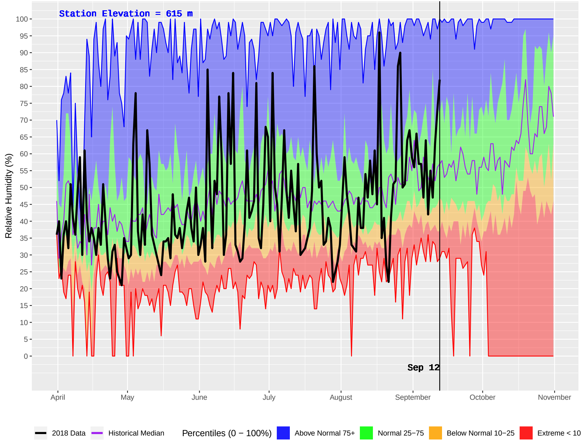
HIXON (187) : Historical (1976–2016) and Current (2018) Daily Relative Humidity
